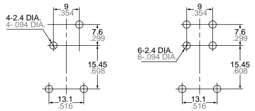
PC board Pattern
